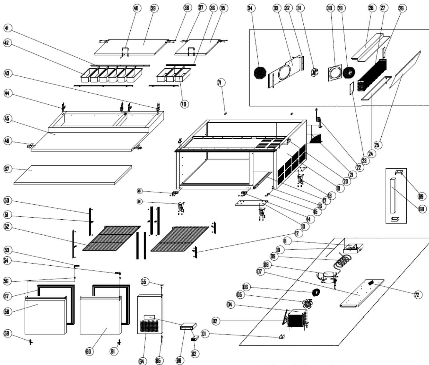
EXPLODE OF KCHPT72.9
